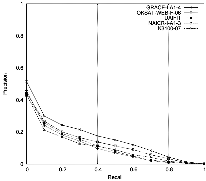
Recall-precision curves for the I-A1 'automatic' and 'DESC-only' runs with considering links (rigid relevance level)
