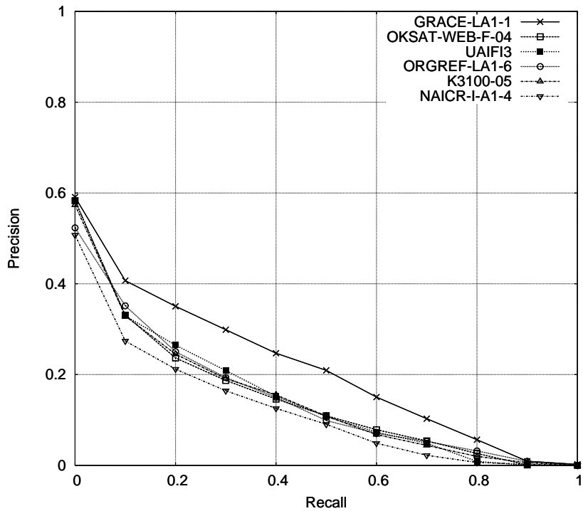
Recall-precision curves for the I-A1 'automatic' and 'TITLE-only' runs with considering links (relaxed relevance level)
