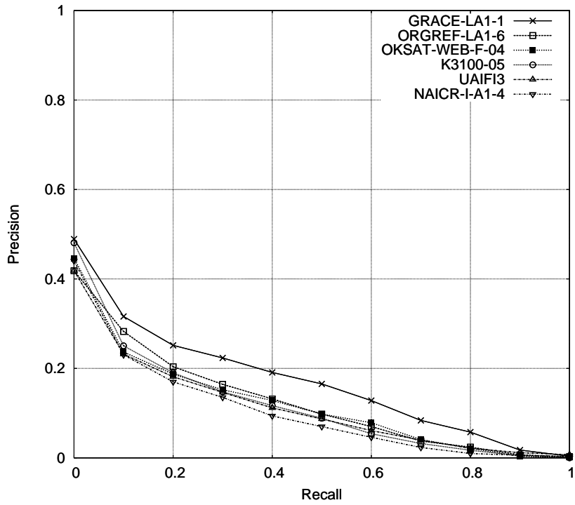
Recall-precision curves for the I-A1 'automatic' and 'TITLE-only' runs with considering links (rigid relevance level)
