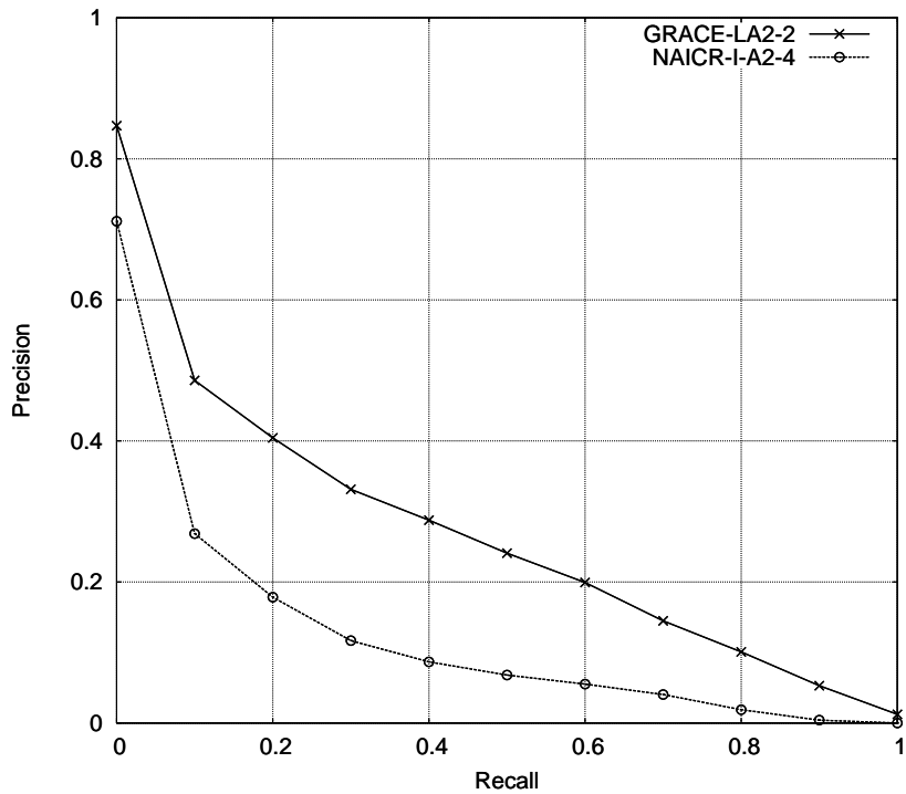
Recall-precision curves for the I-A2 'automatic' and 'TITLE-and-RDOC[1]' runs without considering links (relaxed relevance level)
