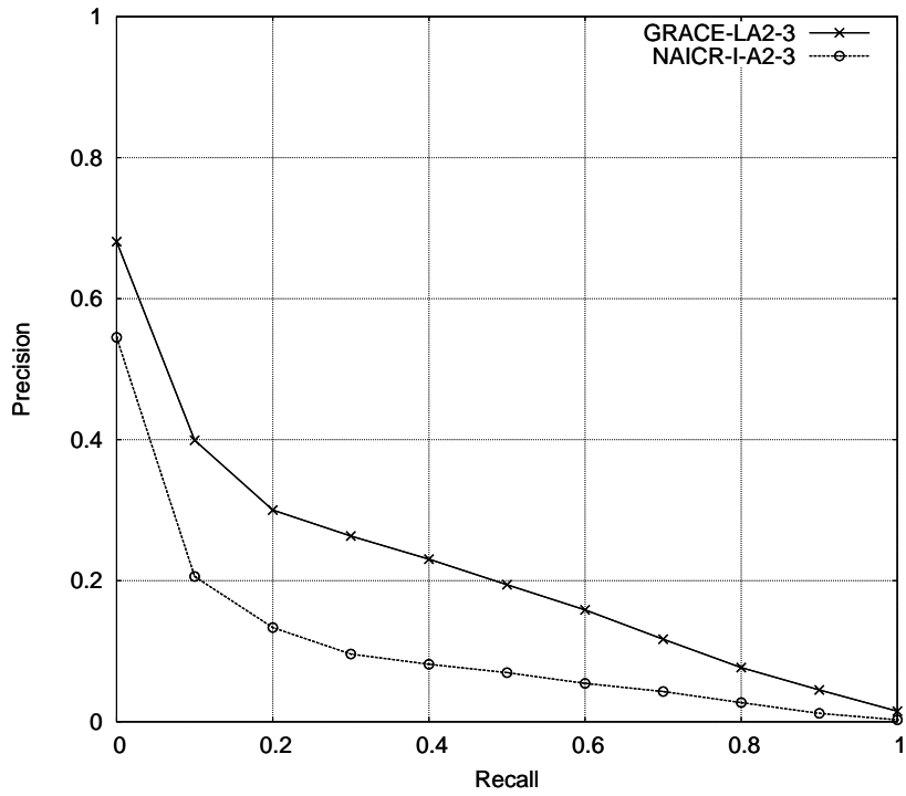
Recall-precision curves for the I-A2 'automatic' and 'TITLE-and-RDOC[1]' runs without considering links (rigid relevance level)
