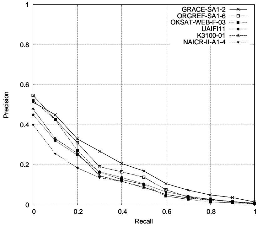
Recall-precision curves for the II-A1 'automatic' and 'TITLE-only' runs with considering links (rigid relevance level)
