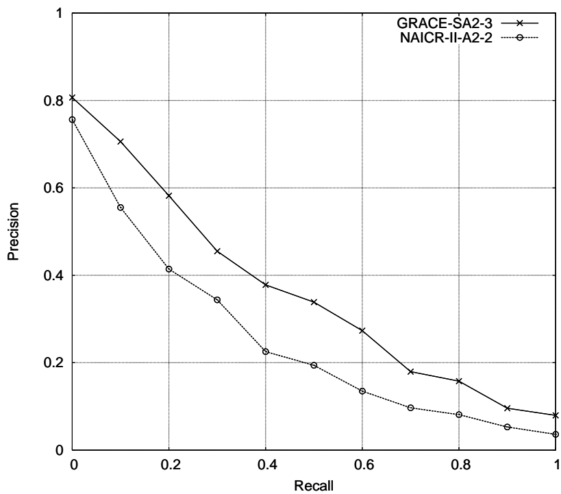
Recall-precision curves for the II-A2 'automatic' and 'TITLE-and-RDOC[1]' runs without considering links (relaxed relevance level)
