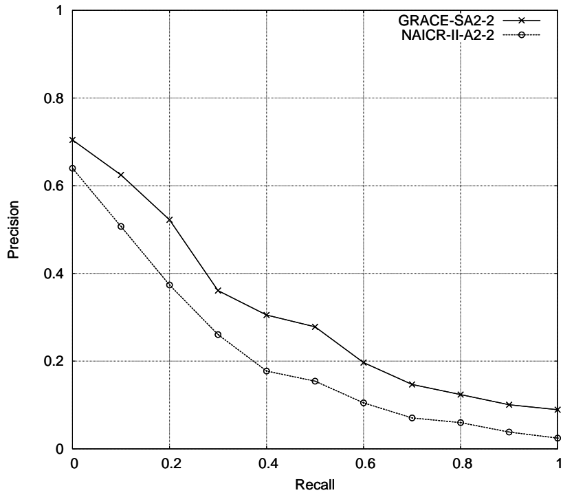
Recall-precision curves for the II-A2 'automatic' and 'TITLE-and-RDOC[1]' runs without considering links (rigid relevance level)
