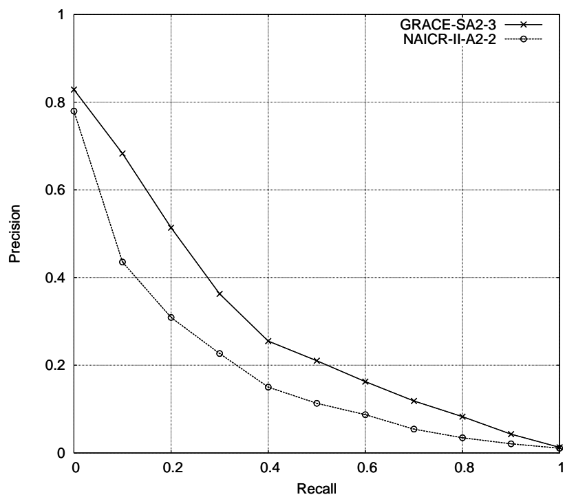
Recall-precision curves for the II-A2 'automatic' and 'TITLE-and-RDOC[1]' runs with considering links (relaxed relevance level)
