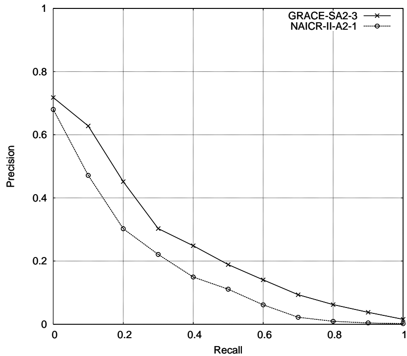
Recall-precision curves for the II-A2 'automatic' and 'TITLE-and-RDOC[1]' runs with considering links (rigid relevance level)
