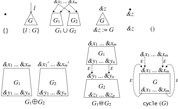
Figure 2. Graph Constructors
