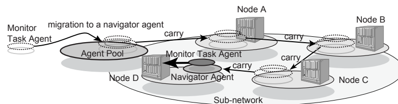
Figure 4: Mobile agent-based management system
