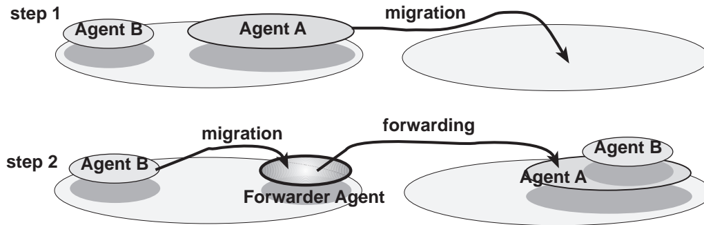
Figure 2: A forwarder agent which transfers its inner agents to other forwarder agents
