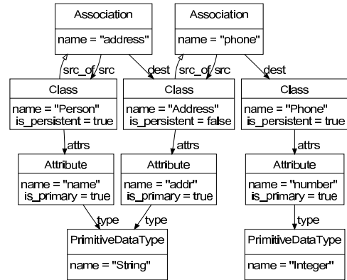
Fig. 2. A Class Diagram
