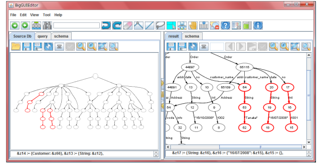
Fig. 3. GUI of GRoundTram
