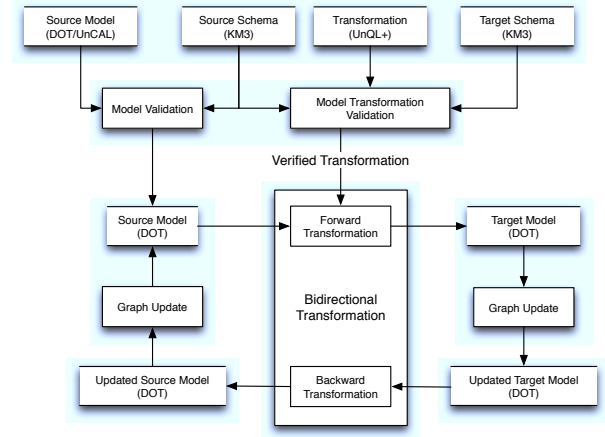
Fig. 1. Overview of GRoundTram
